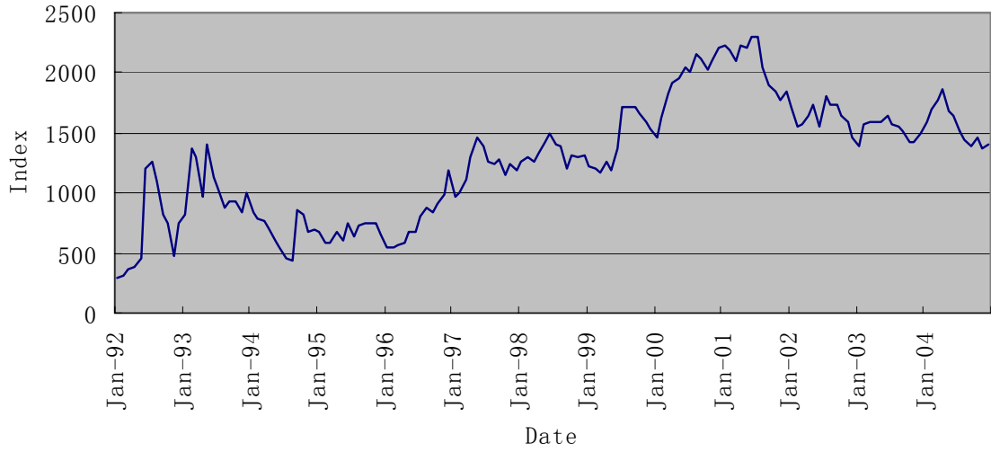
Figure 1A: Time Series Plot of Shanghai A share Index
